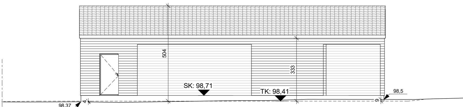
Myn Facade mod syd - vognly
